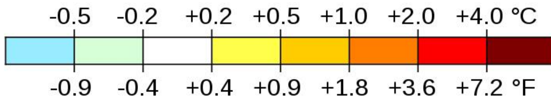
2011-2020 average vs 1951-1980 baseline
